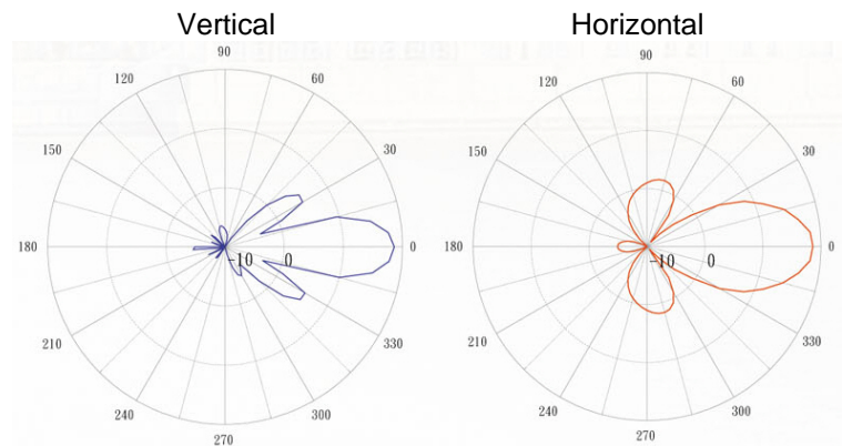
Antenna mounted in vertical polarization
